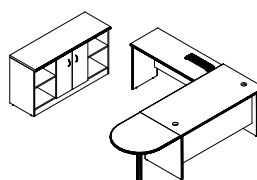
Regus Main Unit - L 1500-1950 D 750-900 Side Unit - L 1200-1500 D 500 Back Unit - L 1350-1650 D 450 Half Round Top - L 750-900 D 750
