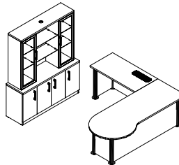
Stellar Main Unit - L 2100-2400 D 750-900 Side Unit - L 1200-1500 D 600 Back Unit - L 1500-1800 D 450 Back Storage - L 1400-1700 D 350
