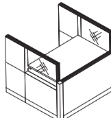
Tele Short L 1200 D 2100 H 1135
