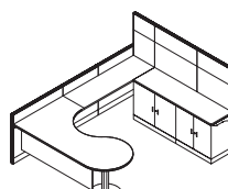
Connect Qube L 1500-1800 D 1050-1200 H 400 Side Panel - H 900 Back Panel - H 1500
