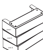
Dynamic Unit 1 - L 1200 D 750 H 400 Unit 2 - L 1200 D 750 H 400 Unit 3 - L 1200 D 750 H 400
