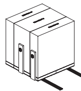
Compactor 2 (Dual Bay) W 1830 D 457 H 1980-2080
