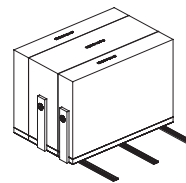
Compactor 3 (Tri Bay) W 2745 D 457 H 1980-2080
